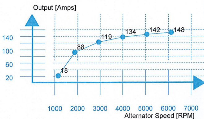
Alternator Performance Curve
